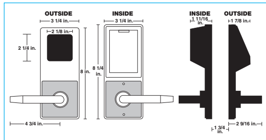
Weather-Resistant Lever with IC Core in 26D DL2800IC/26D
